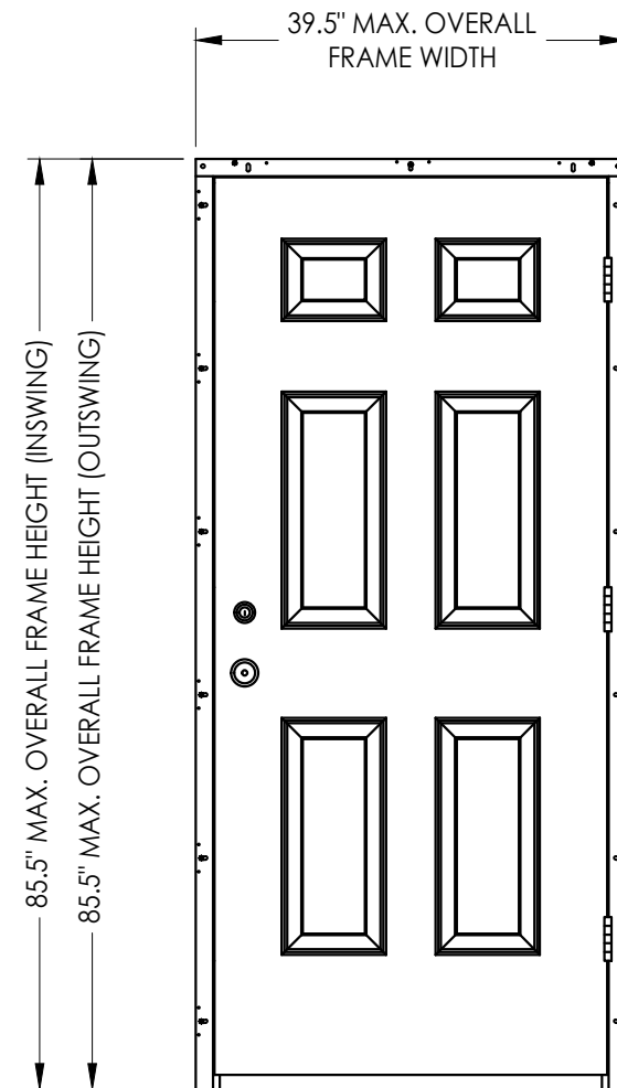
INSWING / OUTSWING
