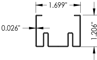
56 BOTTOM RAIL
